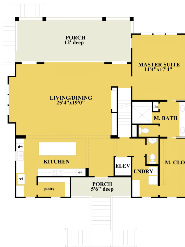
FIRST FLOOR PLAN 1716 HEATED SQUARE FEET
